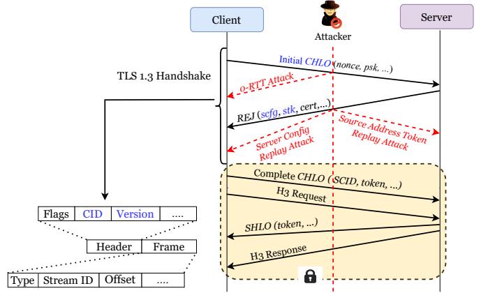
Fig. 2: QUIC connection establishment with attack vectors. The packets or tuples under attack are represented in blue, whereas the attacks are highlighted in red.
